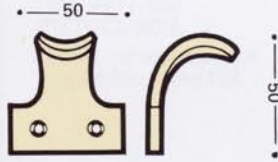
0992C SASH LIFT • cast design
