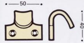
0992 SASH LIFT
