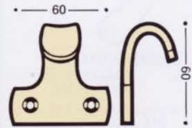
0994C SASH LIFT • heavy cast design
