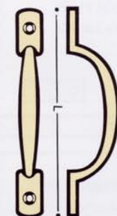
1436 SASH HANDLE lengths L : 102, 127, 152
