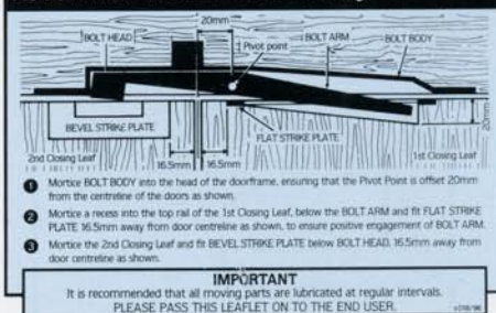
0526 MORTICE RACK BOLT • complete with oval knob turn and coin operated emergency release • to suit doors up to 57mm thick
