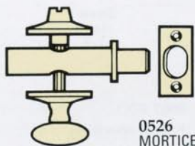
0525 MORTICE RACK BOLT • complete with oval knob turn • to suit doors up to 57mm thick
