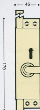
0836 BOLT • lever operation • fitted with 5 lever locking mechanism
