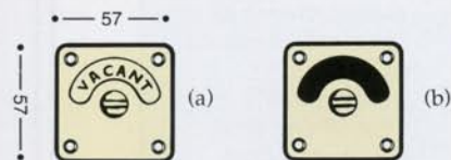
8053 INDICATING BOLT • bolt throws either side for left or right hand application • reversible indicating disc (a) vacant/engaged or (b) red/green • coin operated emergency release
