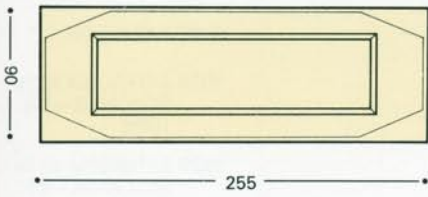
9453 LETTER PLATE • sprung flap
